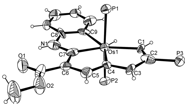
Figure 1. Molecular structure of the cation of 2 (thermal ellipsoids set at 50% probability). The phenyl moieties in \text{PPh}_3 have been omitted for clarity. Selected bond lengths [Å] and angles [°]: Os1–C1 2.175(8), Os1–C4 2.083(10), Os1–C7 1.999(12), Os1–C9 2.151(9), C1–C2 1.347(14), C2–C3 1.389(15), C3–C4 1.450(12), C4–C5 1.369(14), C5–C6 1.390(13), C6–C7 1.457(15), C7–N1 1.400(12), N1–C8 1.427(14), C8–C9 1.371(15); Os1–C1–C2 116.6(8), C1–C2–C3 118.6(11), C2–C3–C4 110.9(9), C3–C4–Os1 120.0(7), C4–Os1–C1 73.8(4), Os1–C4–C5 122.2(7), C4–C5–C6 113.0(10), C5–C6–C7 108.8(10), C6–C7–Os1 123.8(7), C7–Os1–C4 71.9(4), Os1–C7–N1 123.0(9), C7–N1–C8 110.8(10), N1–C8–C9 115.4(10), C8–C9–Os1 116.1(8), C9–Os1–C7 74.5(4).
